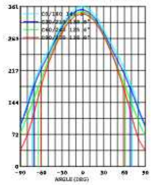
LUMINOUS INTENSITY DISTRIBUTION
